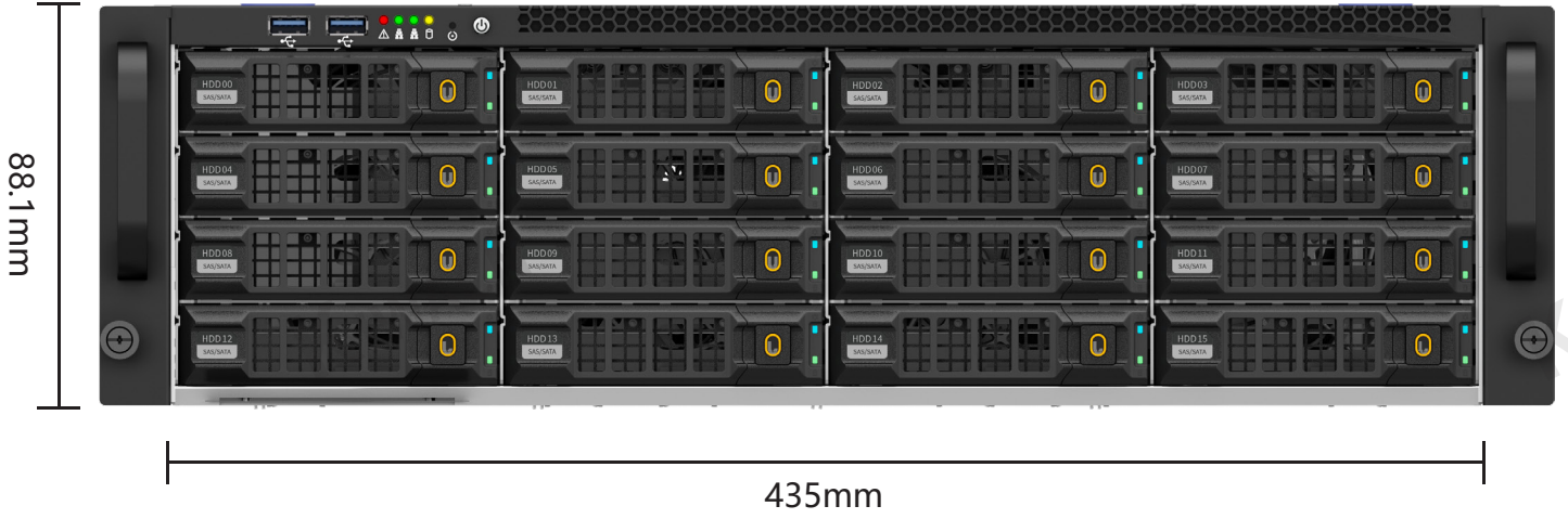
Front View (Dimensions)
